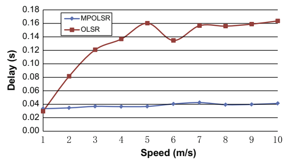
Fig. 6. Average end-to-end delay of MP-OLSR and OLSR in a scenario for 81 nodes and 4 sources.
