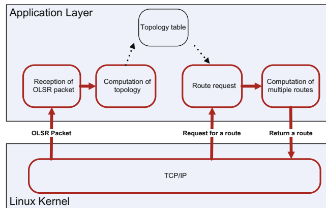
Fig. 15. Implementation of MP-OLSR on Linux.
