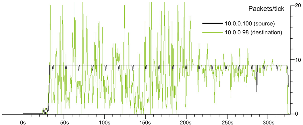
Fig. 23. Wireshark trace of UFTP source and destination nodes, 81 nodes MP-OLSR ad hoc network.
