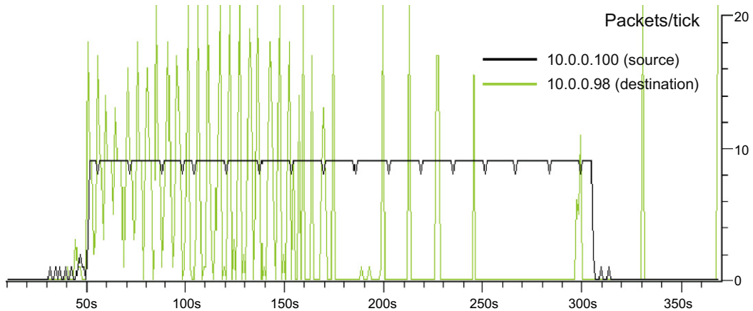
Fig. 22. Wireshark trace of UFTP source and destination nodes, 81 nodes OLSR ad hoc network.
